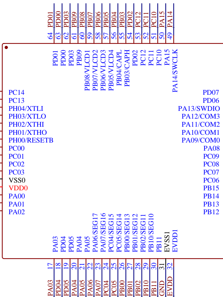
U1 BAT32G127GH64FB
